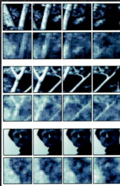
Fig 1. A comparison of the real images shown to the cats (top in each row) with the reconstructed visual obtained by decoding the LGN neuronal activity (bottom in each row) Figure taken from Stanley, Li and Dan (1999)
