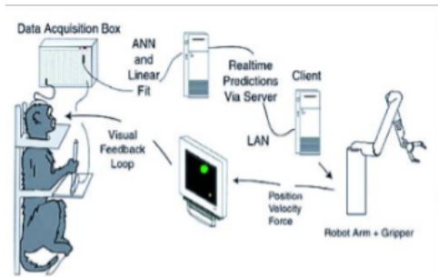
Fig 2. The setup used by Carmena et al. (2003) to get monkeys to learn how to control a robotic arm simply through their thoughts.
